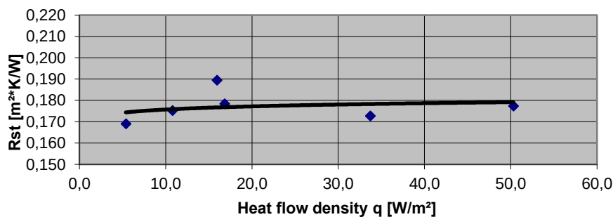
Total surface resistance R_{st}
