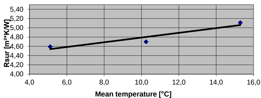
Thermal resistance around the frame R_{sur}
